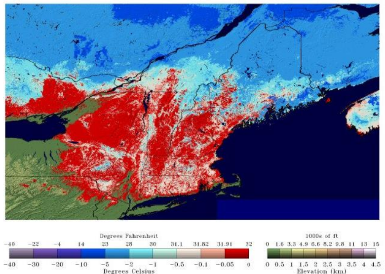
Average Snowpack Temperature 24-Hour Average Ending 2017-02-23 06 UTC
